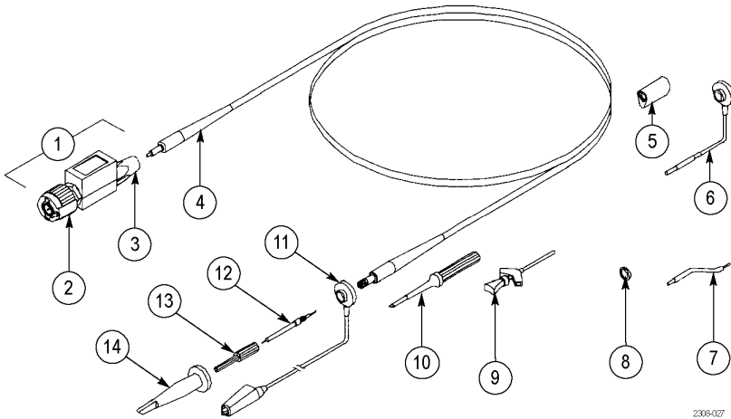
Standard Accessories
